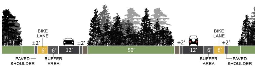
Figure 10 - Alternative 3 cross sections.
