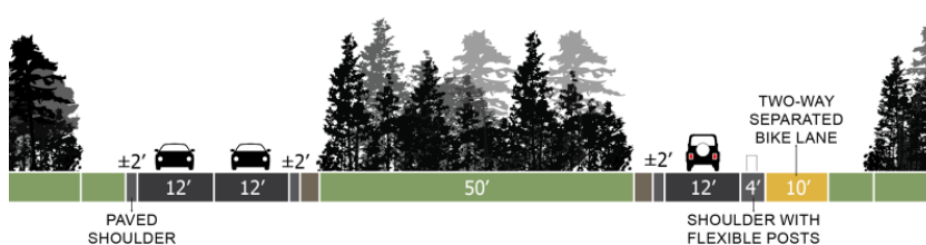
Figure 9 - Alternative 2 cross sections.
