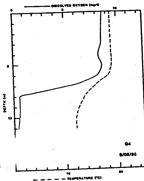
DISSOLVED OXYGEN AND TEMPERATURE VERSUS DEPTH
