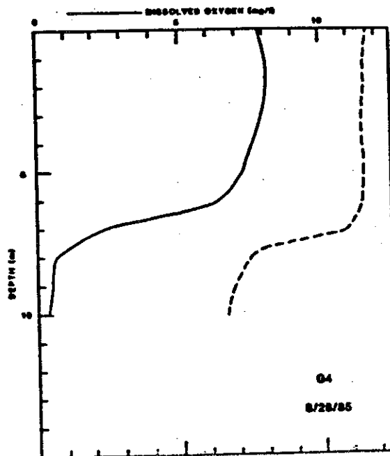
DISSOLVED OXYGEN AND TEMPERATURE VERSUS DEPTH
