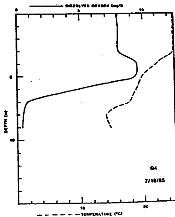
DISSOLVED OXYGEN AND TEMPERATURE VERSUS DEPTH
