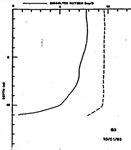
DISSOLVED OXYGEN AND TEMPERATURE VERSUS DEPTH
