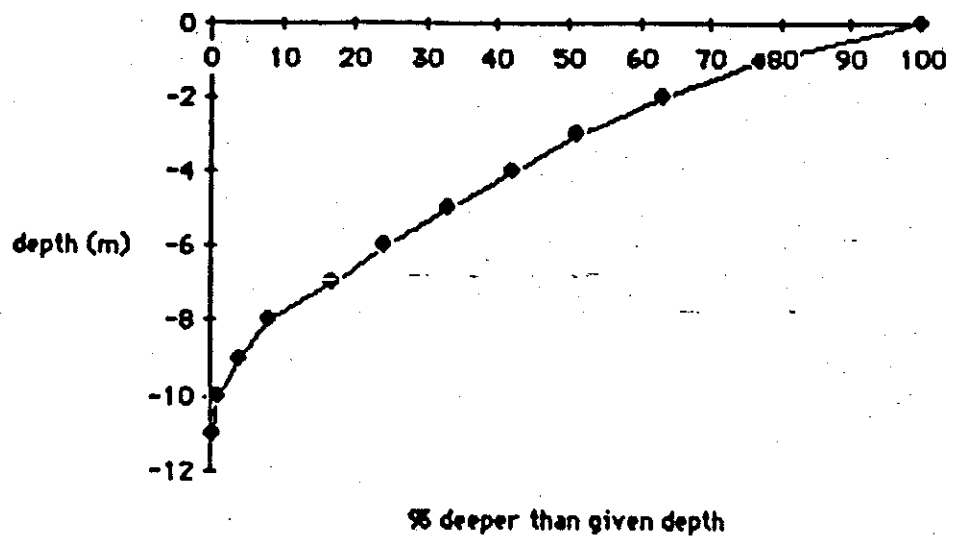
FIGURE 3 Great Pond Hypsographic Curve
